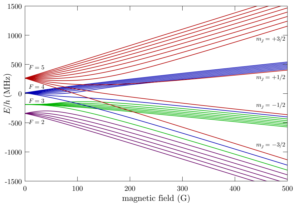
Figure 6: Cesium 6^2P_{3/2} ( D_2 excited) level hyperfine structure in an external magnetic field. The levels are grouped according to the value of F in the low-field (anomalous Zeeman) regime and m_j in the strong-field (hyperfine Paschen-Back) regime.
