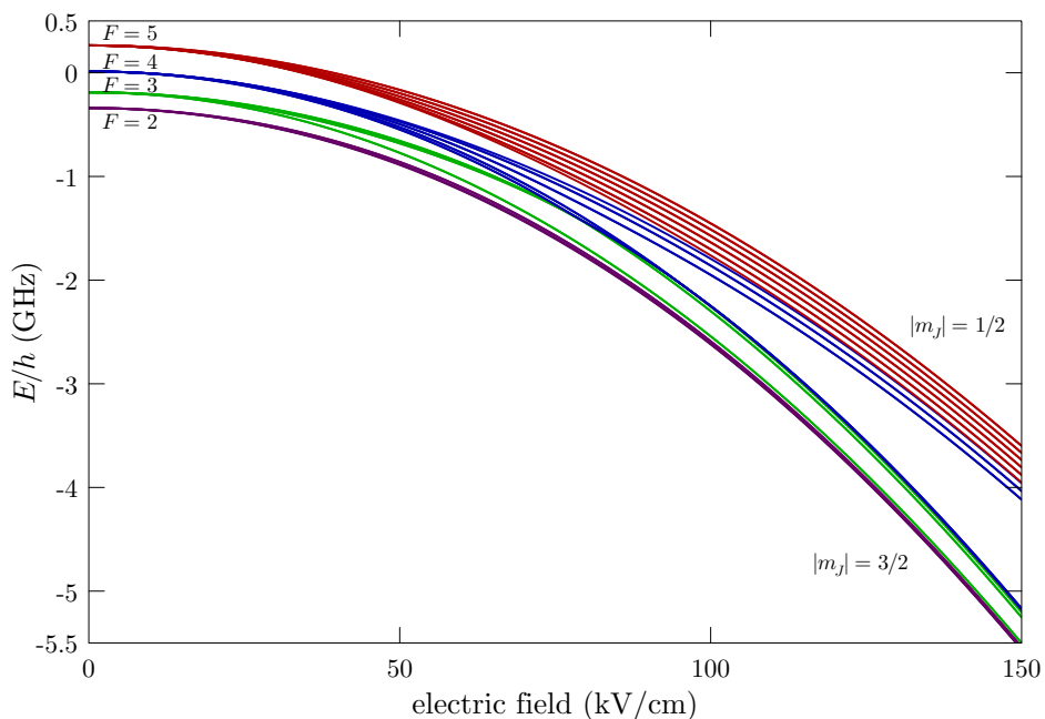
Figure 7: Cesium 6^2P_{3/2} ( D_2 excited) level hyperfine structure in a constant, external electric field. The levels are grouped according to the value of F in the low-field (anomalous Zeeman) regime and |m_j| in the strong-field ("electric" hyperfine Paschen-Back) regime. Levels with the same values of F and |m_F| (for a weak field) are degenerate.
